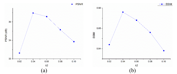
Fig. 26. Denoising performances with different values of \lambda_2 . (a) PSNR. (b) SSIM.
